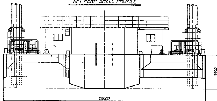
AFT PERP SHELL PROFILE
